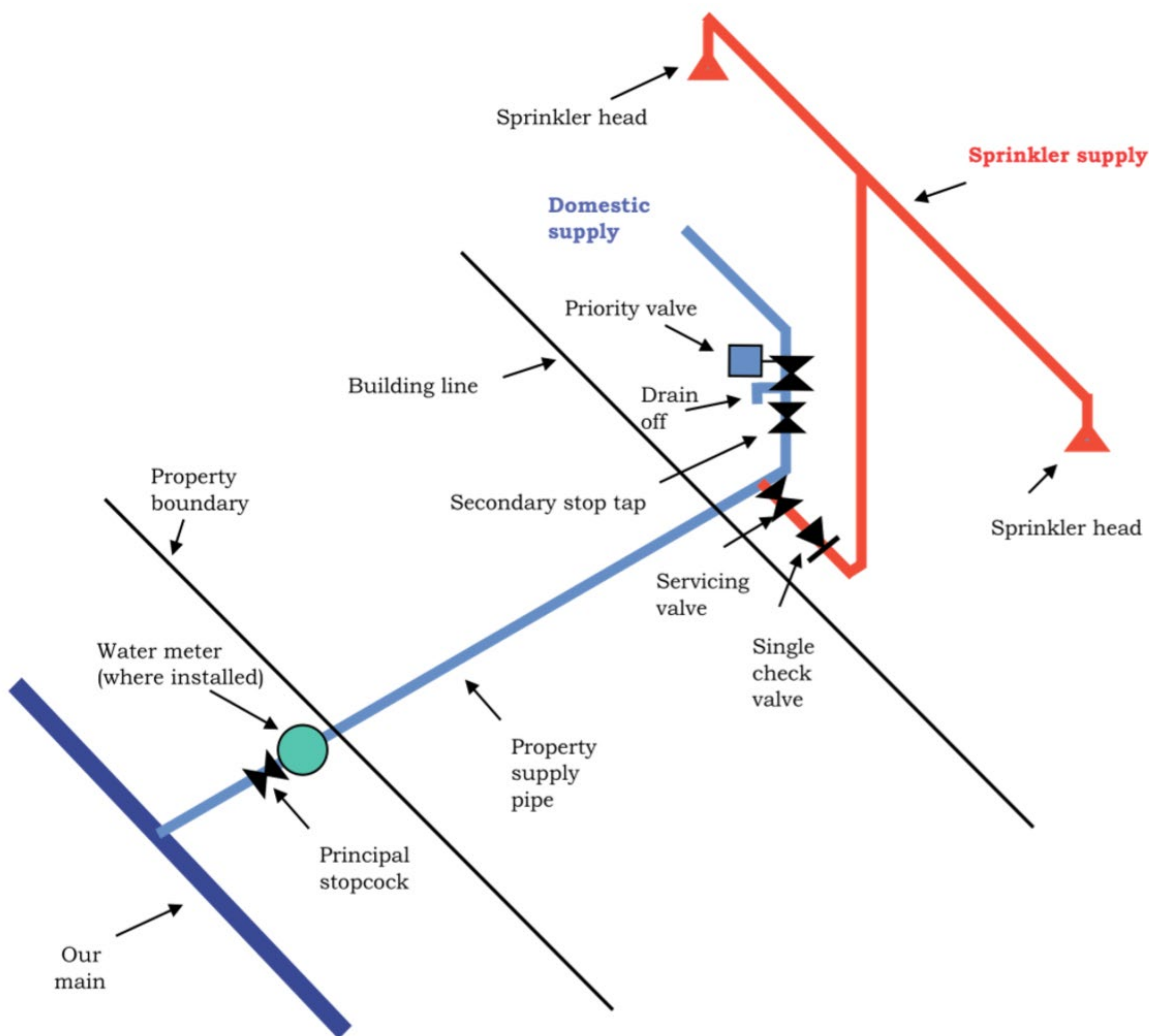
[Example of a direct feed sprinkler schematic]
